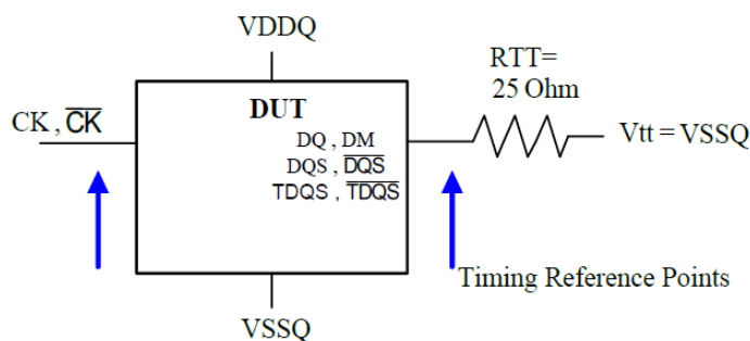
ODT Timing Reference Load
