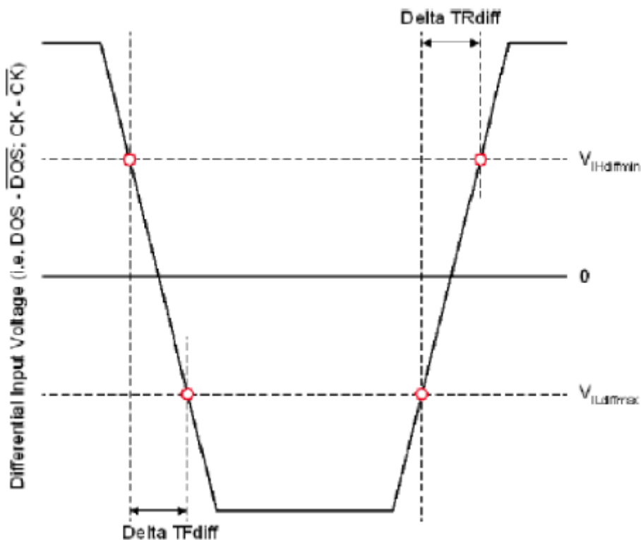
Differential Input Slew Rate Definition for DQS, \overline{\text{DQS}} and CK, \overline{\text{CK}}
